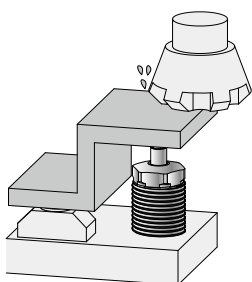
To avoid chattering of a thin workpiece
