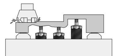
To support an uneven workpiece
